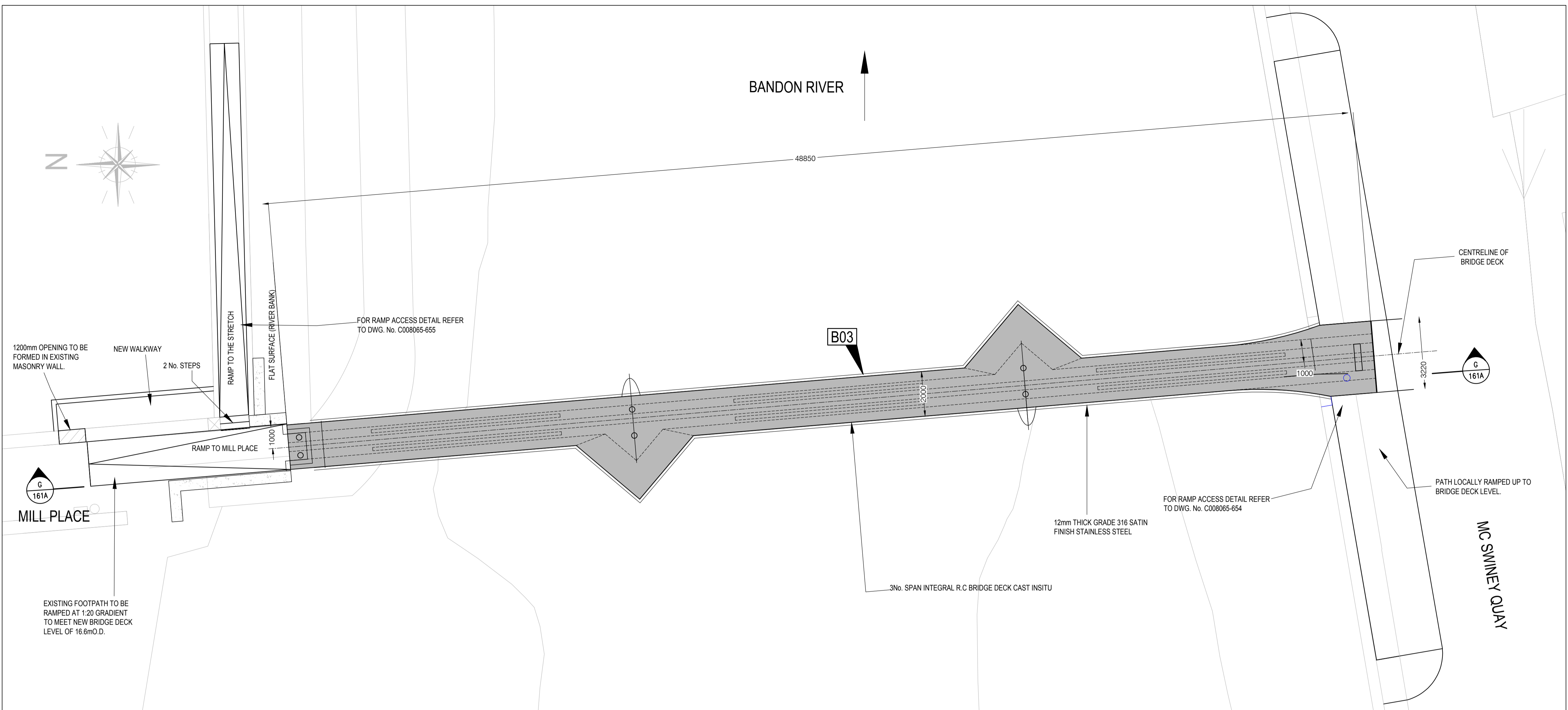
BANDON RIVER FOOTBRIDGE GENERAL ARRANGEMENT SCALE 1:100
